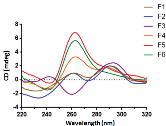
Figure 2. CD spectra of anion exchange chromatography fractions of d(G4C2)_2 . The concentration of each fraction was 20 \mu M .
